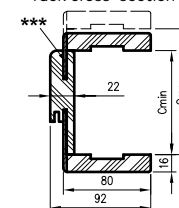
rack cross-section
