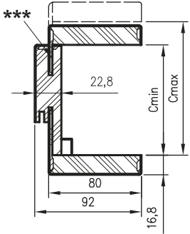
beam cross-section
