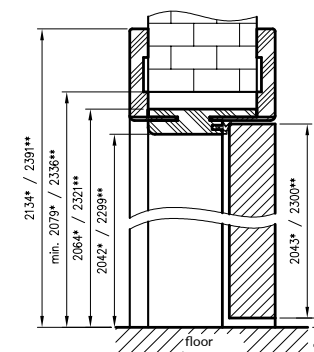
vertical cross-section
