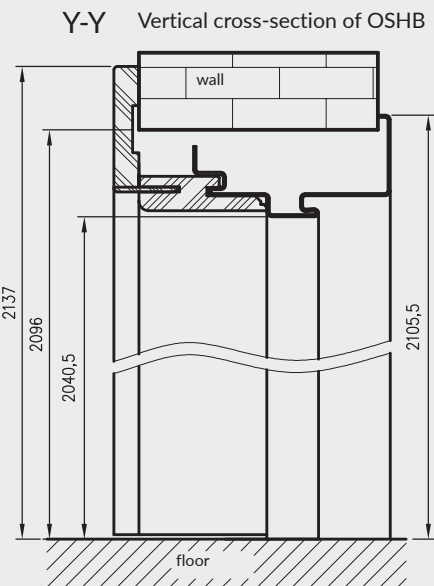
hybrid steel non-rebated door frame profile
