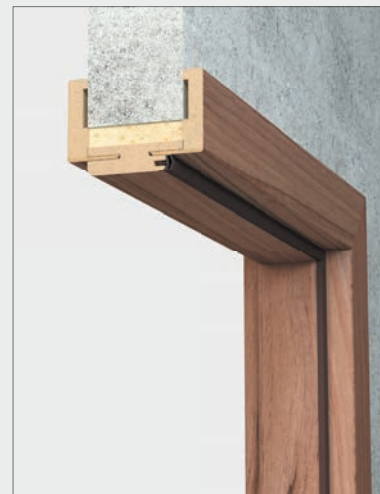
OR (adjustable rebated door frame) with T63
