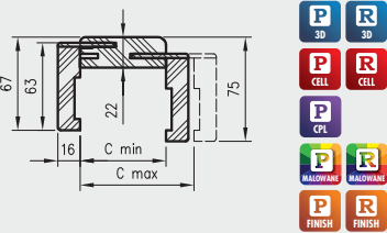
tunnel cross-section with T63 architrave
