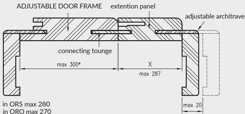
options of the width of panels cross-section
