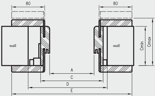
D - required width of wall opening
