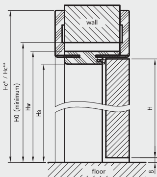
ORB vertical cross-section
