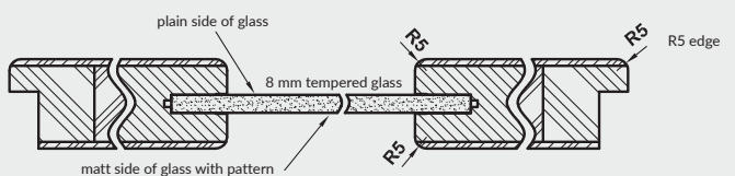
Horizontal cross-section of VETRO B5, B10-B11
