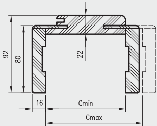
OR cross-section with T80 architrave
