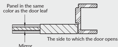
Estra 10 door in the "reverse" variant
