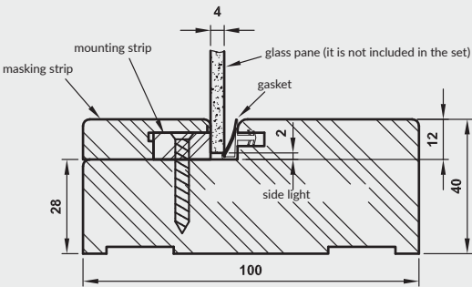
Dimensions of transom lights/sidelights
