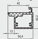
DRE profile for non-rebated outward opening doors
