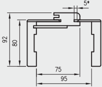
ORB cross-section 075
