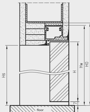
DRE profile for non-rebated outward opening doors
