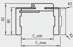
ORB cross-section 075
