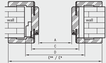
OR/ORC horizontal cross-section
