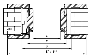
OR horizontal cross-section
