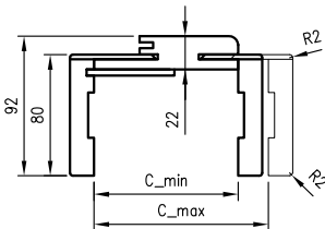
ORB cross-section 095-300
