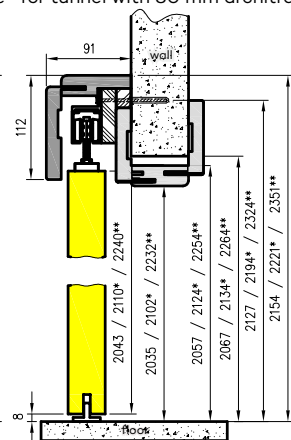
NT - vertical cross-section for tunnel with 80 mm architrave
