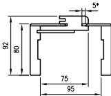
ORB cross-section 075
