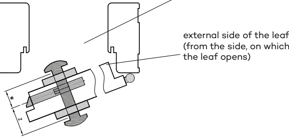
fig. selection of cylinder insert dimension with door knob
