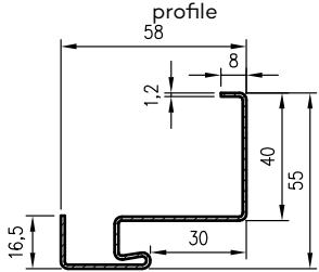
small angular steel door frame
