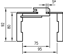
ORB cross-section 075
