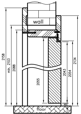
vertical cross-section of ORO
