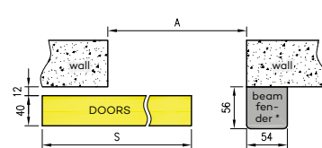
NS - horizontal cross-section (left system)
