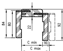
tunnel cross-section with T63 architrave
