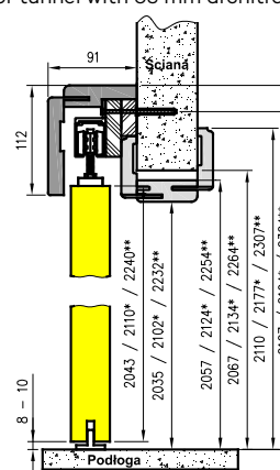
NT - vertical cross-section for tunnel with 63 mm architrave
