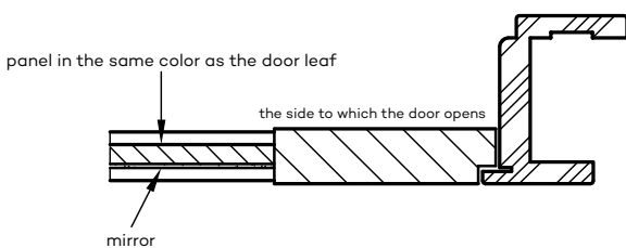
ESTRA 10 door with inverted rebate in the "Reverse" variant
