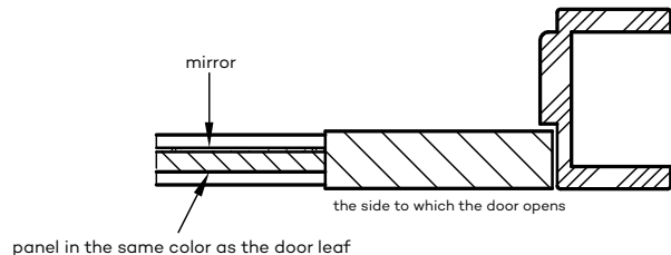
ESTRA 10 doors, non-rebated or rebated, in the "Reverse" variant
