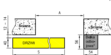
double leaf sliding system
