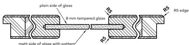
Horizontal cross-section of VETRO A5, B5, D1 door
