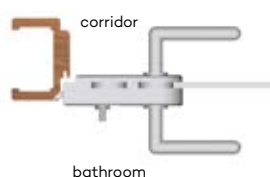
fig. 1 right door leaf /blockade outside
