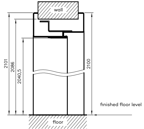
Vertical section of the OSRB
