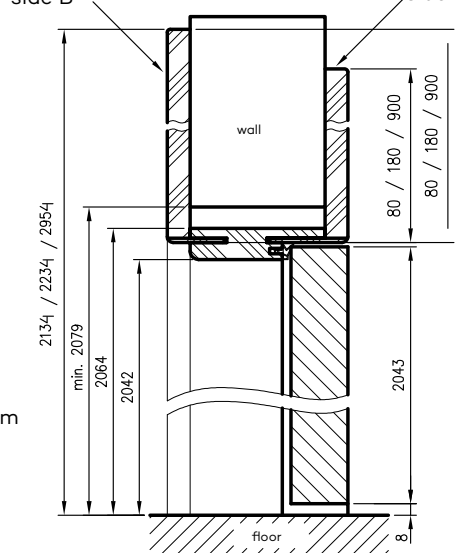
side B A-A Vertical section side A
