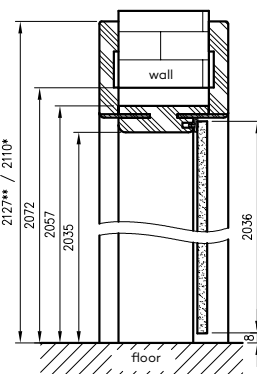
vertical cross-section of glass doors with ORC (adjustable door frame for glass doors)
