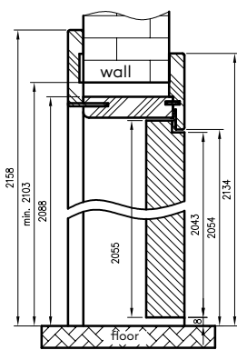
vertical cross-section of ORO
