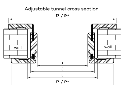
tunnel cross-section with T63 architrave
