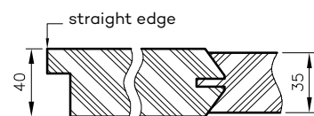
Horizontal cross-section of ELSA
