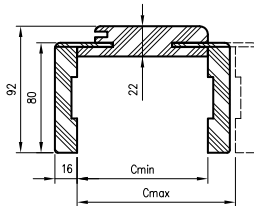
OR/ORC cross-section with T80 architrave
