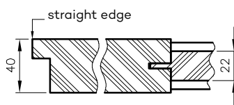
Horizontal cross-section of ELSA
