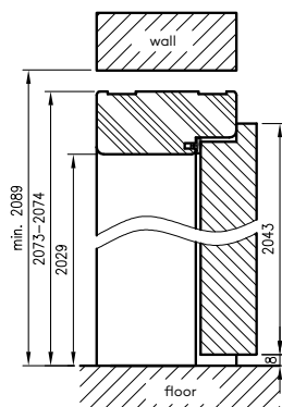
OP vertical cross-section for rebated door leaf
