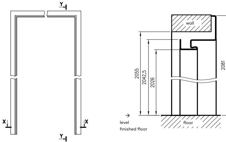
Dimensions for single leaf doors
