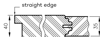
Horizontal cross-section of Nestor
