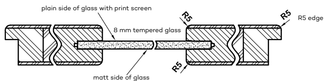
Horizontal cross-section of VETRO A5, B5, D1 door
