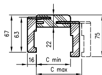
tunnel cross-section with T63 architrave
