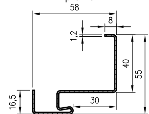
small angular steel door frame profile
