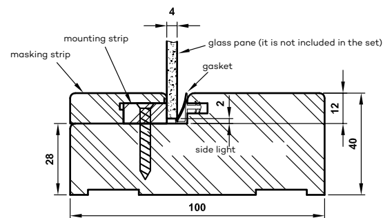
Dimensions of transom lights/side lights
