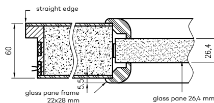
Fire resistant door leaf Olimp EI60
