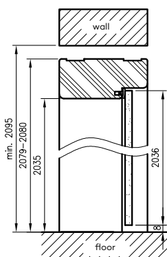
OP vertical cross-section for glass doors
