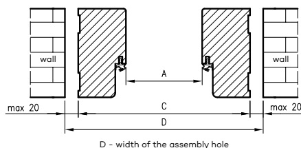
horizontal cross-section of door frame in the wall
