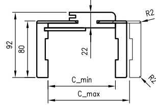
ORB cross-section 075
