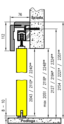
NS - vertical cross-section
