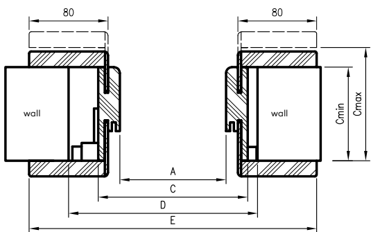
B-B Horizontal cross-section
