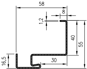
small angular steel door frame profile
