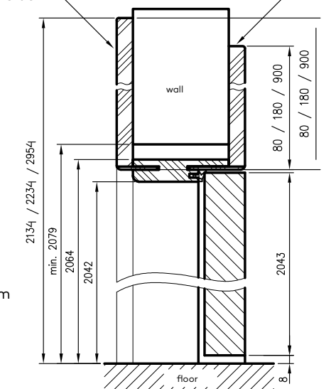
A-A Vertical cross-section side B side A
