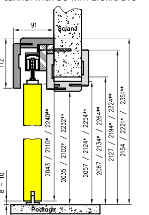
NT - vertical cross-section for tunnel with 80 mm architrave
