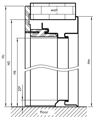
OSH STAND dimensions for double leaf doors
