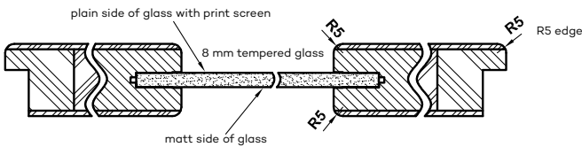
Horizontal cross - section of VETRO A5, B5, D1 door
