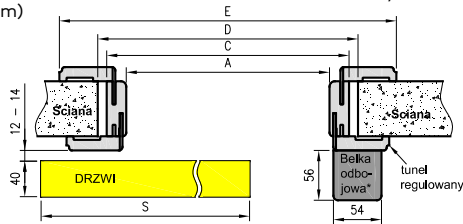
NT - horizontal cross-section (left system)
